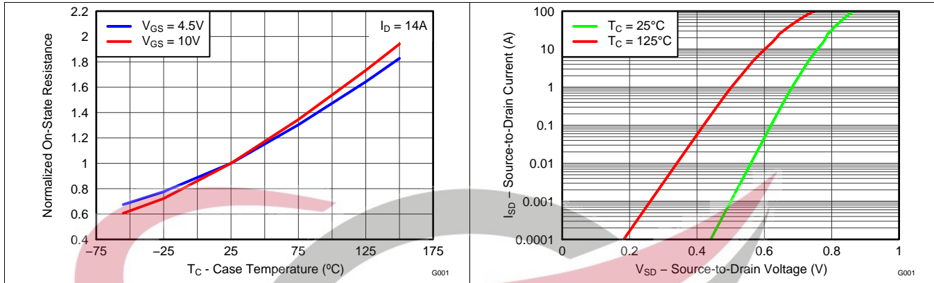
Figure 8. Normalized On-State Resistance vs Temperature
